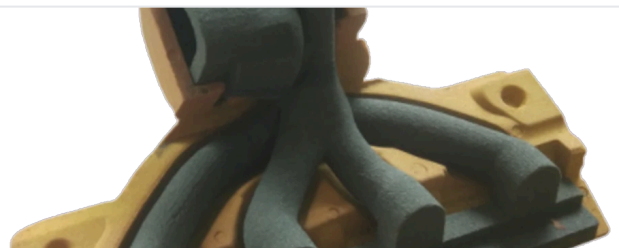
Exhaust manifold core — thin-wall geometry without tooling
